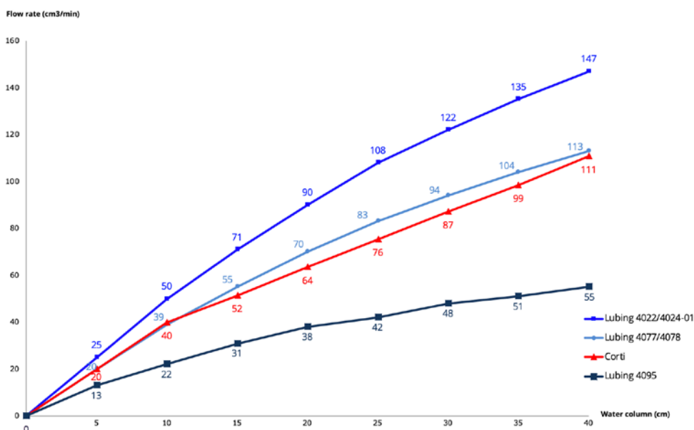
FLOW CHART (TRIGGER PINS LIFTED 7 MM (0.2756 inch) (3 MM (0.1181 inch) FOR LUBING 4095))
