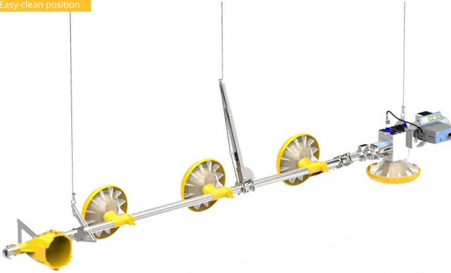
Easy-clean position
