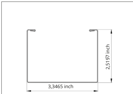
Standard trough
