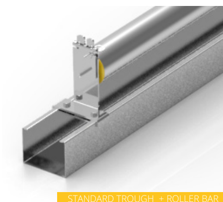
STANDARD TROUGH + ROLLER BAR
